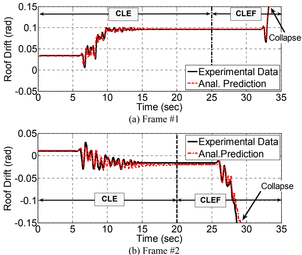
Fig. 3. Roof drift histories for both frames during CLE and CLEF testing phases together with analytical predictions
