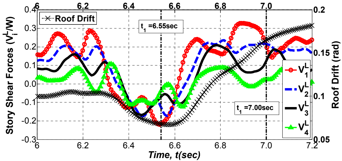
Fig. 5. Effective story shear force histories for Frame #1, CLEF
