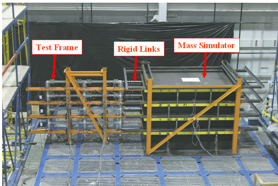
Fig. 1. Test setup on the NEES earthquake simulator
