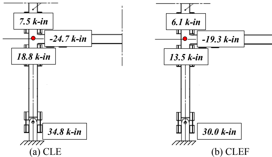
Fig. 9. Moment distribution of exterior subassembly at first story during CLE and CLEF
