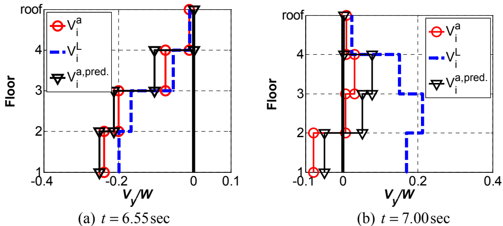
Fig. 6. Story shear force distributions along the height of Frame #1 during CLEF for selected times together with analytical predictions
