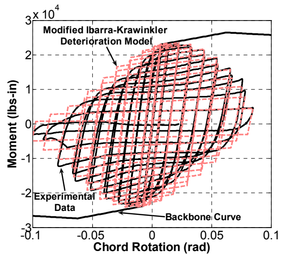
(b) calibrated hysteretic response
