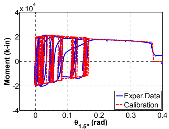
(b) first floor beam at exterior corner
