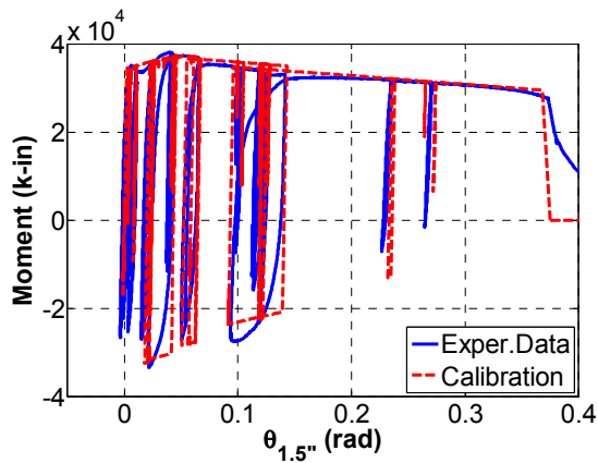
(a) Exterior column at base
