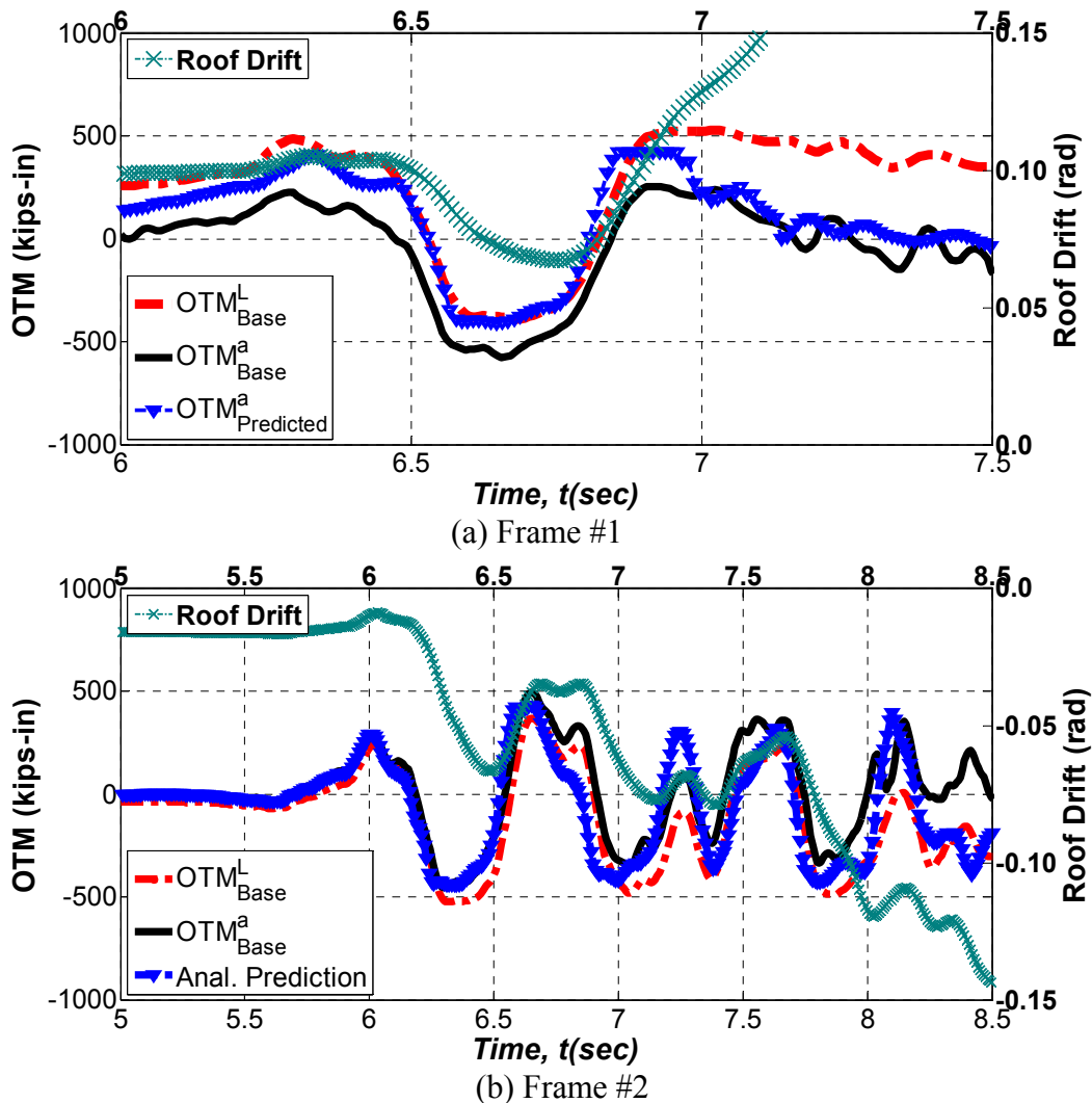
Fig. 7. Overturning moment history at base for both frames, CLEF
