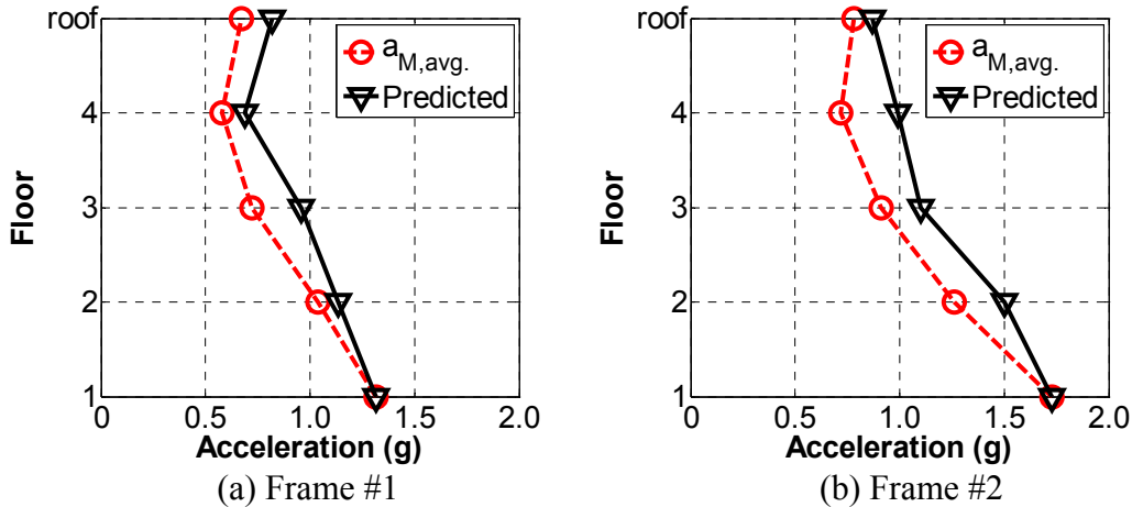
Fig. 4. Peak absolute acceleration along the height of both frames during CLE
