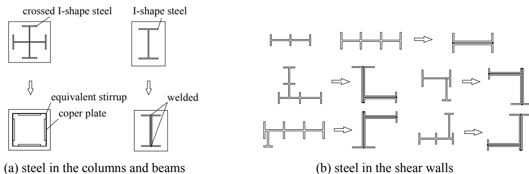
Fig. 5 Simplification of steel section
