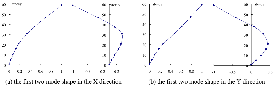
Fig. 8 The first two modal shapes in the two directions
