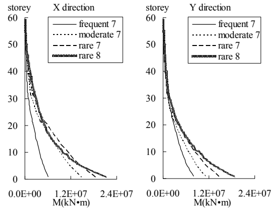
Fig. 11 Envelopes of the overturning moment
