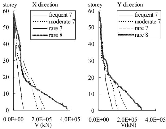
Fig. 10 Envelopes of the shear force
