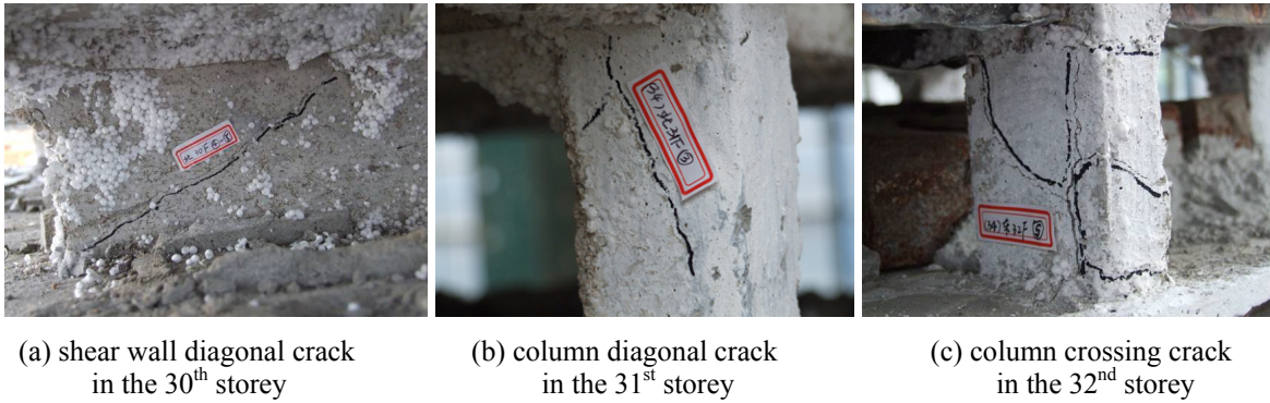
Fig. 7 Failure pattern of the model structure
