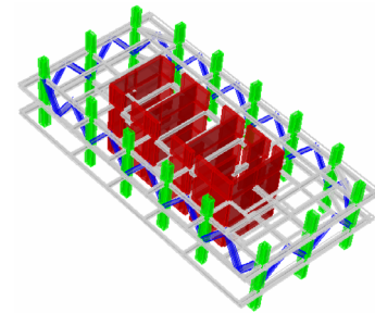
Fig. 2 Belt truss in the 47 th floor
