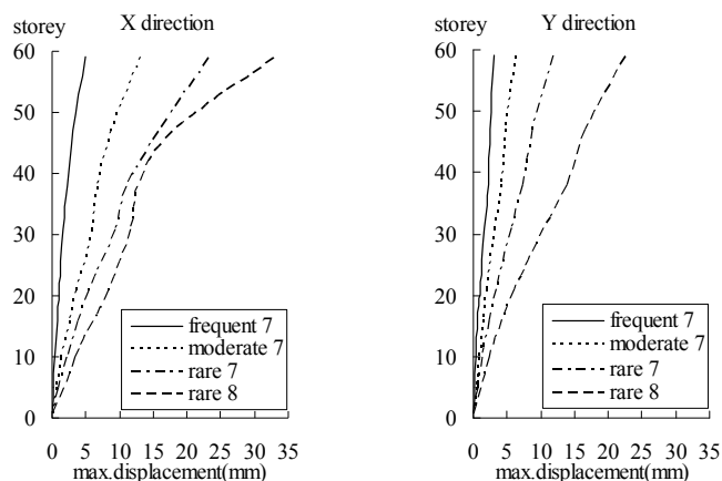
Fig. 9 Displacement response envelopes of the model structure
