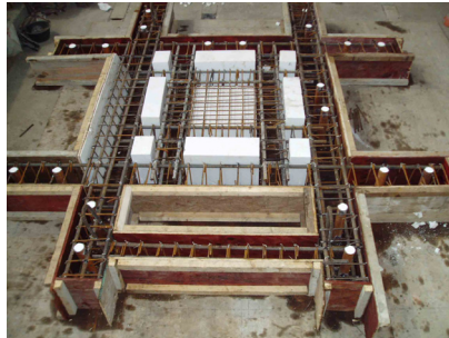
(a) base of the model
