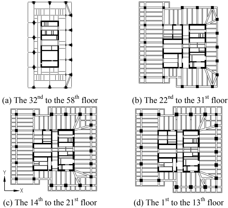
Fig. 1 Typical plan layouts of each part
