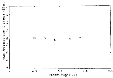
6 EARTHQUAKES ALL SITES BL 60 BARS 100 CM/SEC T=0.01 SEC
