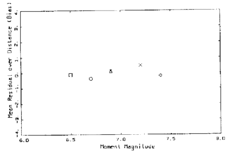
6 EARTHQUAKES ALL SITES BL 60 BARS 100 CM/SEC T=2.00 SEC
