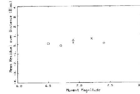
6 EARTHQUAKES ALL SITES BL 60 BARS 100 CM/SEC T=3.00 SEC
