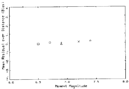
6 EARTHQUAKES ALL SITES BL 60 BARS 100 CM/SEC T=0.50 SEC
