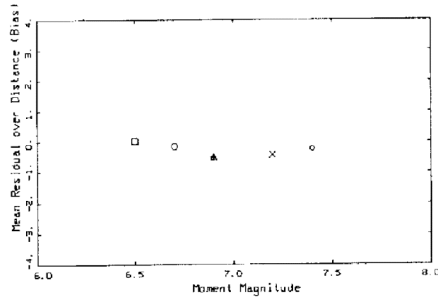
6 EARTHQUAKES ALL SITES BL 60 BARS 100 CM/SEC T=0.20 SEC
