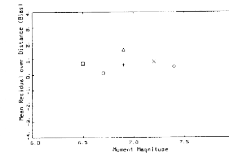
6 EARTHQUAKES ALL SITES BL 60 BARS 100 CM/SEC T=10.0 SEC
