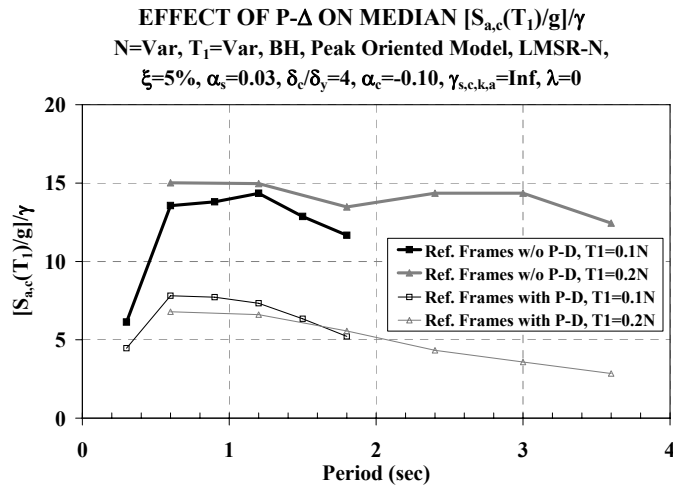
Fig. 4. Effect of P-Delta on Median Collapse Capacity of Reference Moment Frames ( [S_{a,c}(T_1)/g]/\gamma is the median R_{\mu} factor at collapse)
