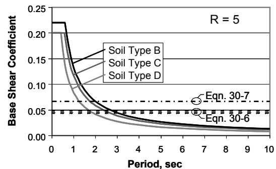
Figure 2. UBC-97 required design base shear for typical development site in San Francisco.
