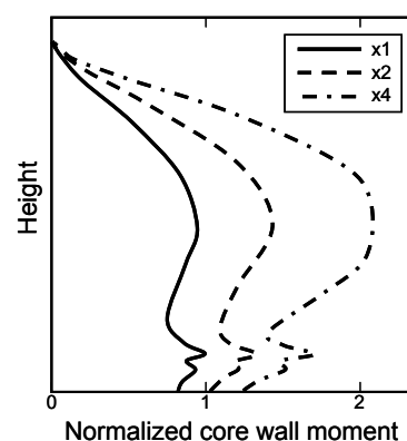
Figure 5. Variation of mean core wall moments for M7 ground motions multiplied by factors of 1, 2, and 4.
