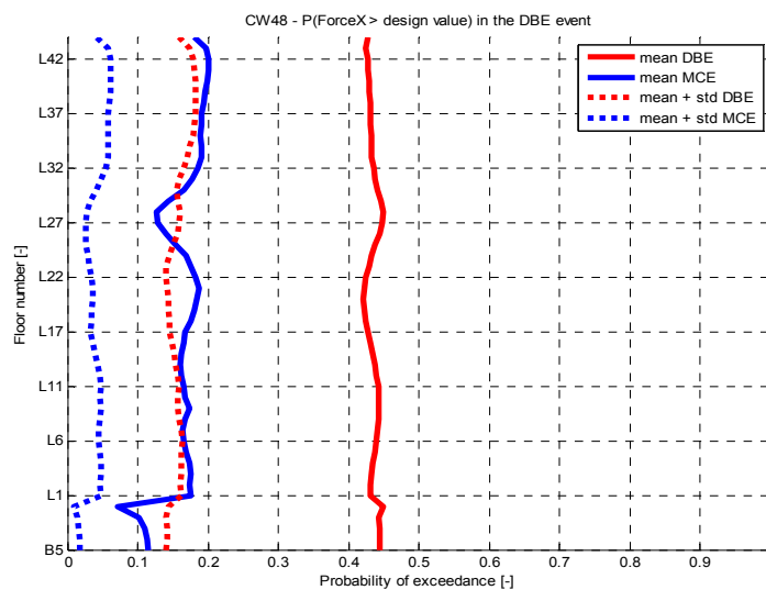
Figure 8. Probability of exceeding the design shear for ground shaking at the 475-year uniform hazard level value, for design shears based on the mean from DBE, mean from MCE, or mean plus one standard deviation for DBE and MCE.
