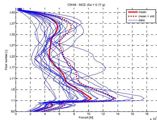
Figure 7. Story shears in a case study core-wall building, from nonlinear response history analysis, for ground motions scaled so the first-mode spectral acceleration matches the uniform hazard level value at the MCE hazard level.
