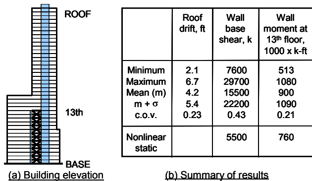
Figure 6. Building elevation and summary of nonlinear dynamic and nonlinear static analysis results. Nonlinear static analysis results are for inverted triangular floor acceleration pattern.
