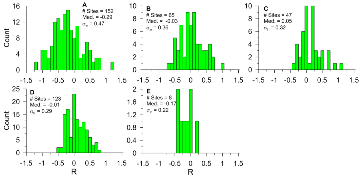
Figure 3.13 Residuals of V_{s30} from estimates based on the geotechnical proxy (Geomatrix 3 rd letter) using the methods of Chiou et al. (2008). Based on V_{s30} measurements and V_{sz} - V_{s30} relations.
