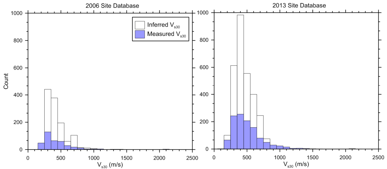
Figure 3.2 Histograms of measured and inferred V_{s30} at the recording station sites in both the 2006 and 2013 site databases.
