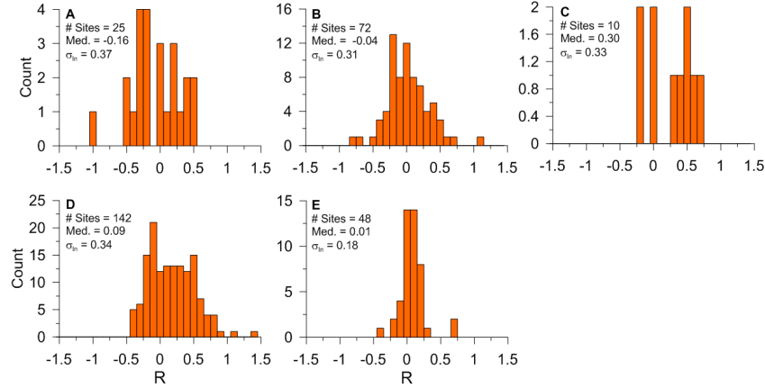
Figure 3.19 Residuals of V_{s30} from estimates based on elevation-based method within GMX 3rd letter categories using the methods of Chiou and Youngs (2008a). Based on V_{s30} measurements and V_{sz} - V_{s30} relations for Taiwan data.
