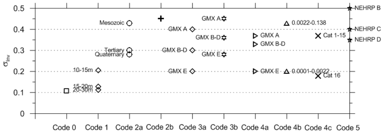
Figure 3.28 Recommend dispersion of V_{s30} in natural log units when derived from various information sources.
