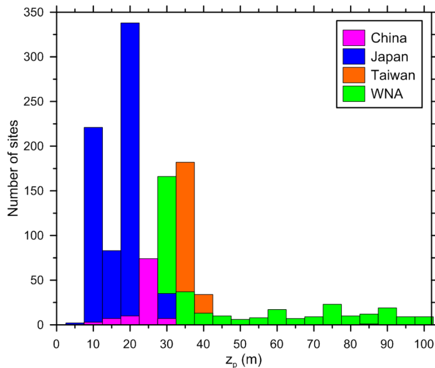
Figure 3.4 Histogram of profile depth bins by region. Profile depths for Japan extend up to 365 m, but are concentrated at 100 m in the figure. Note that there is one station with z_p = 82 m in Japan.
