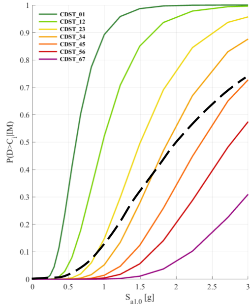
Figure 2. Preliminary fragility model comparisons between the g2F fragility models (colorful lines) and HAZUS models (black lines) for transverse column responses in an Era 3 bridge with flexural failure
