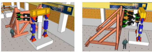
Experimental setup for the planned hybrid simulation tests
