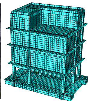
Full-scale base-isolated building specimen: photo (left) on the E-Defense shake table (courtesy T. Okazaki, Hokkaido Univ.); high-fidelity finite element model (right).
