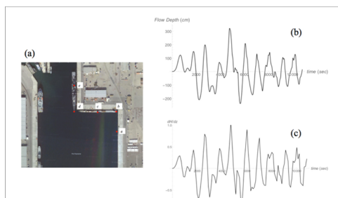
Quantification of uncertainties using the Data Explorer for the quay wall of the port of Port Hueneme.
