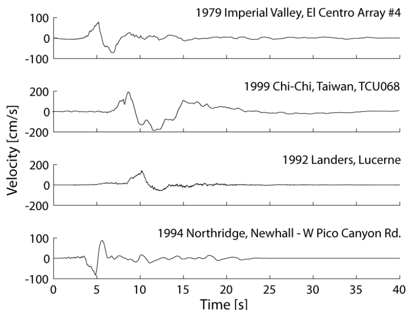
Figure 3.9 Strike-normal velocity time histories of four ground motions from Set #3.
