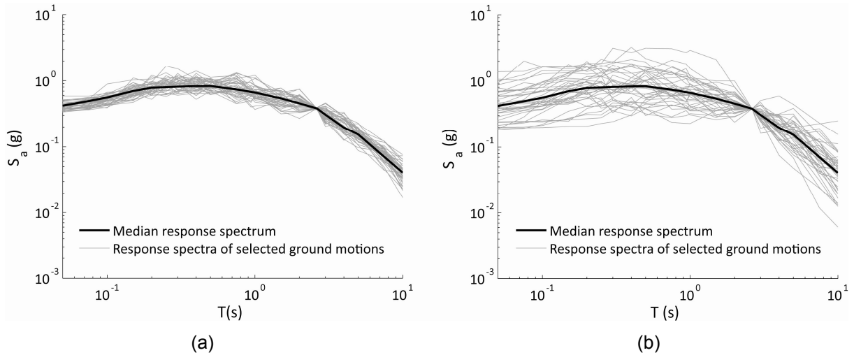
Figure 2.4 Response spectra of 40 selected ground motions for \varepsilon = 2 and T^* = 2.63 sec; (a) Method 1 matched target response spectrum mean, and (b) Method 2 matched target response spectrum mean and variance.
