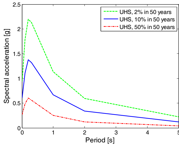
Figure 3.15 Uniform hazard spectra for the Oakland site.
