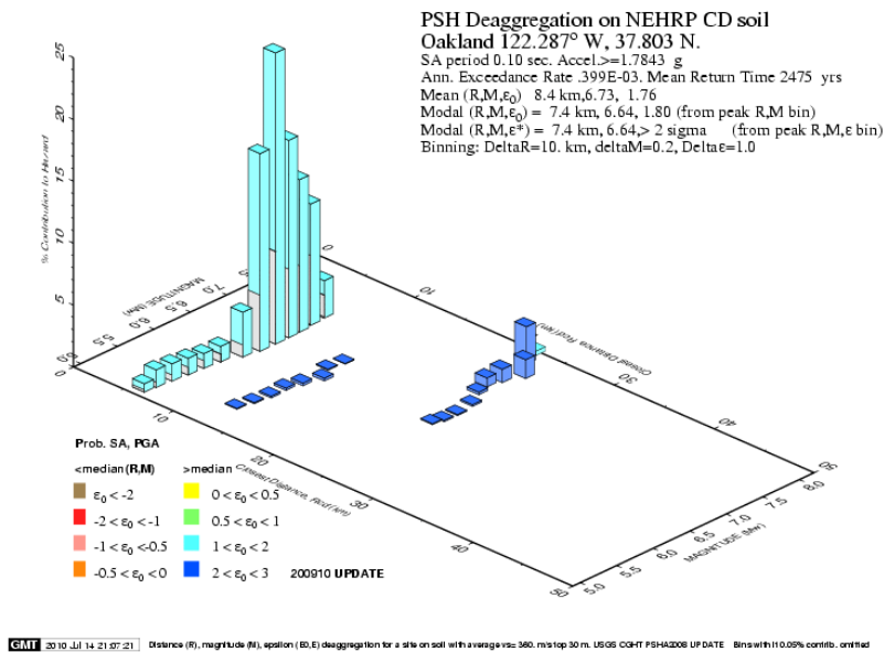
Figure 3.16 Deaggregation plot for S_a(0.1 \text{ sec}) exceeded with 2% probability in 50 years The largest contribution is from the Hayward fault at 7 km, with a small contribution from M>7 earthquakes on the San Andreas fault (figure from USGS 2008).
