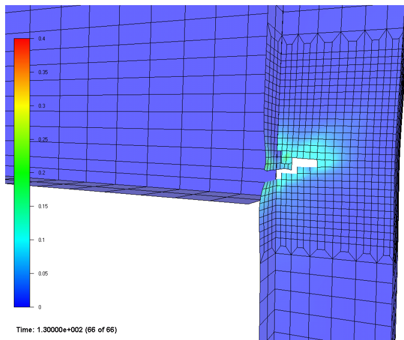
Figure 5.32 Damage and fracture of beam-column connection
