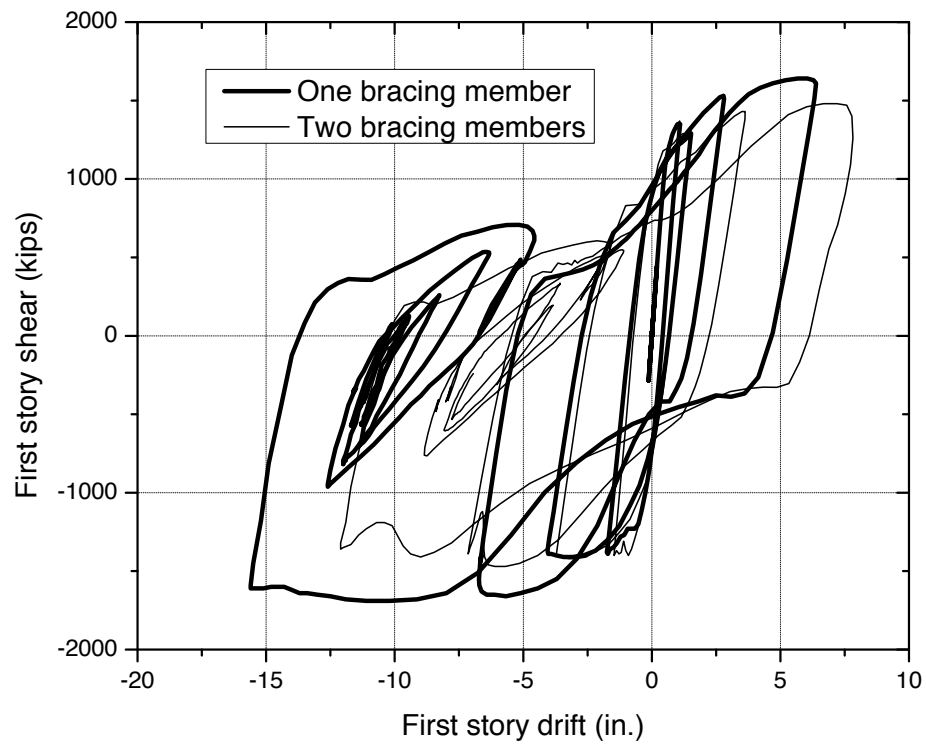
Figure 6.24 Comparison of first-story hysteretic loops
