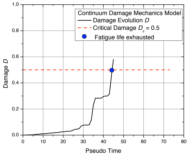
Figure 3.7 Damage evolution of CDM model
