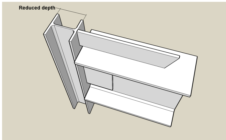
Figure 6.14 Details of column: reduced depth
