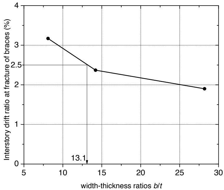
Figure 6.2 Interstory drift ratios to failure versus width-thickness ratios
