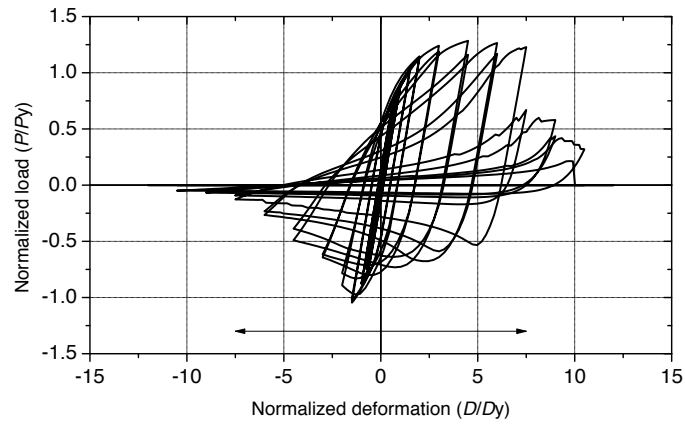
(b) 2 cycles per deformation level
