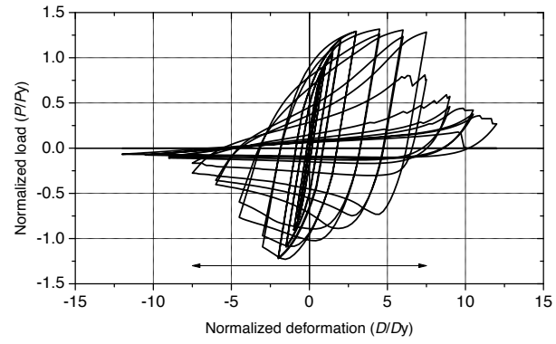
(a) KL/r = 32
