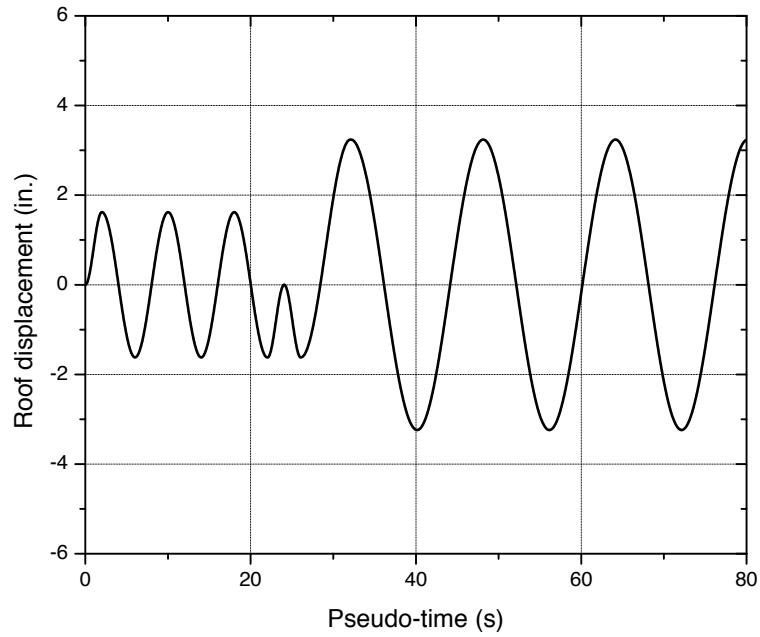
(a) Displacement history
