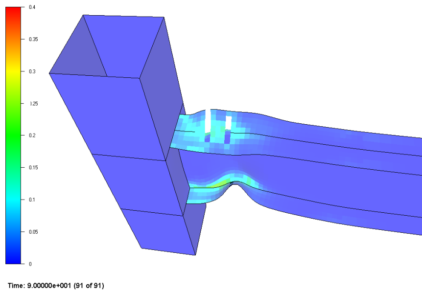
Figure 5.30 Predicted fracture in top flange
