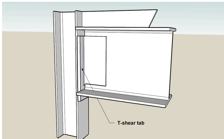
Figure 6.20 Details of reinforcement: T-shear tab
