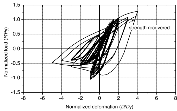
(b) b/t = 15.9 , pass
