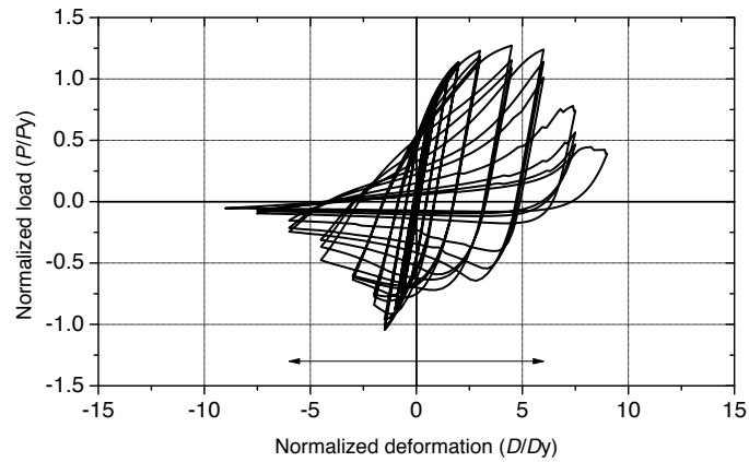
(c) 3 cycles per deformation level
