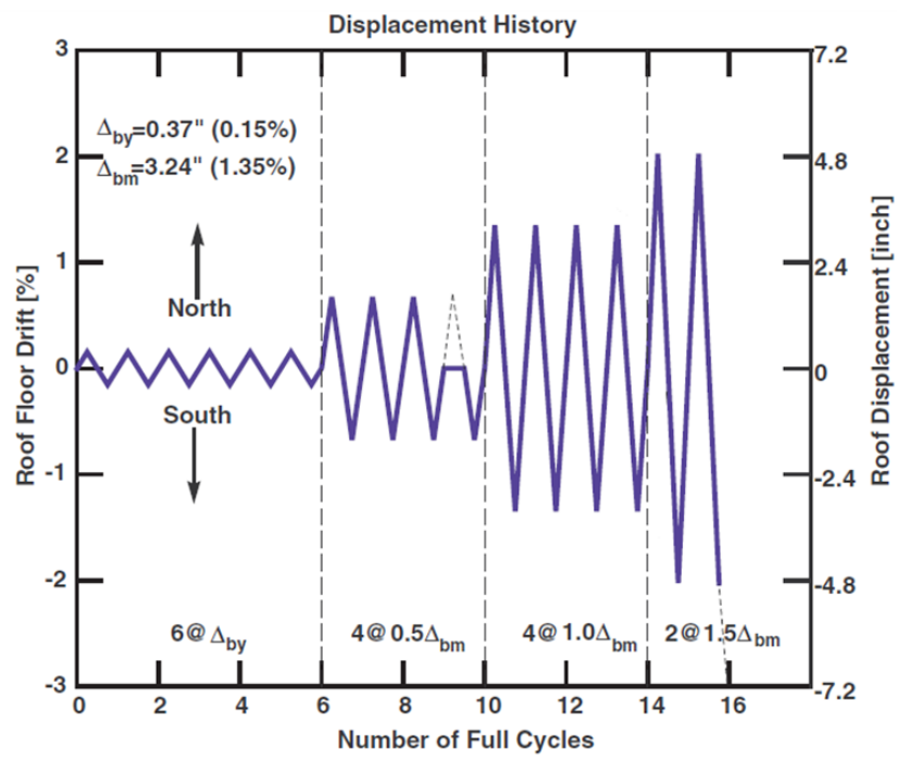
Figure 2.4 Target roof displacement history of SCBF test (Uriz, 2005)
