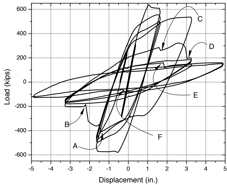
Figure 2.8 Base shear versus roof lateral displacement (Uriz, 2005)
