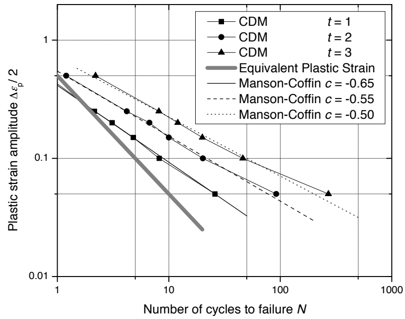
Figure 3.9 Manson-Coffin plot of CDM model
