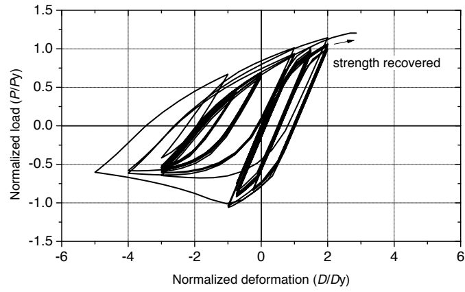
(a) b/t = 15.3 , pass
