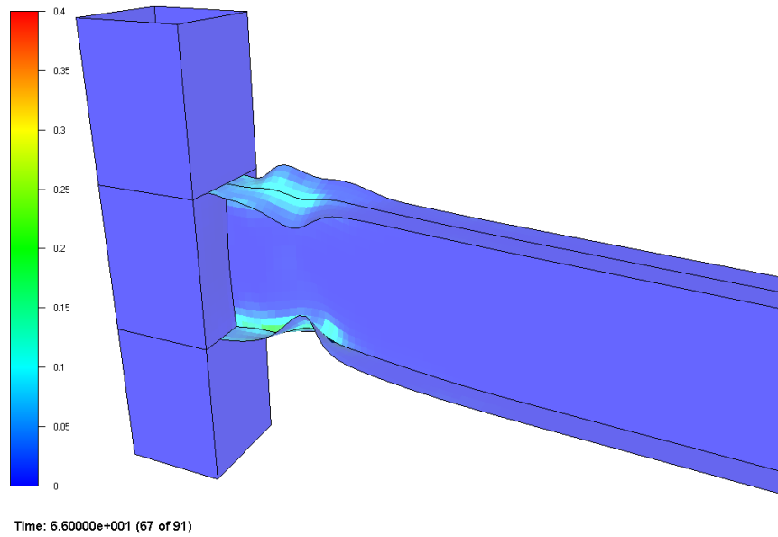
Figure 5.29 Predicted local buckling and damage
