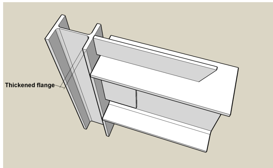
Figure 6.16 Details of column: thickened flange
