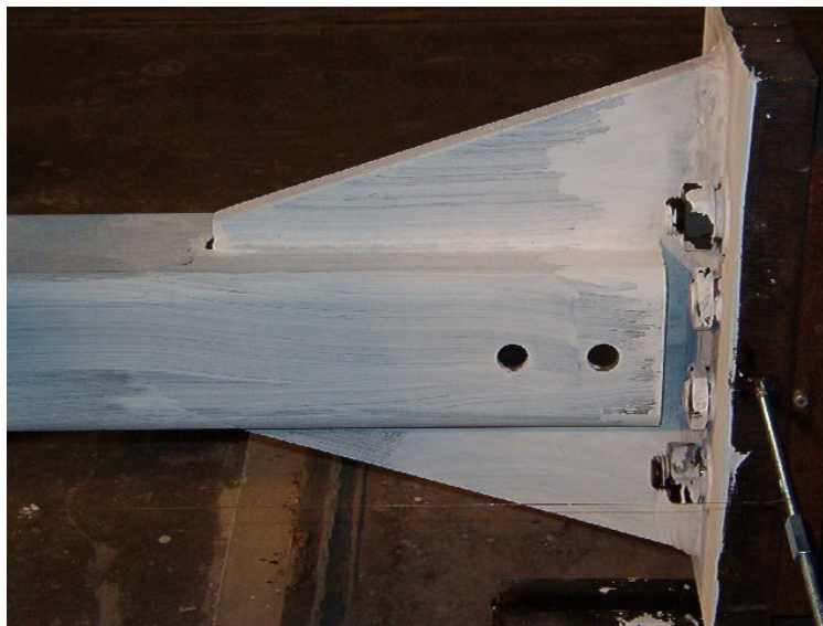
(b) End connection
