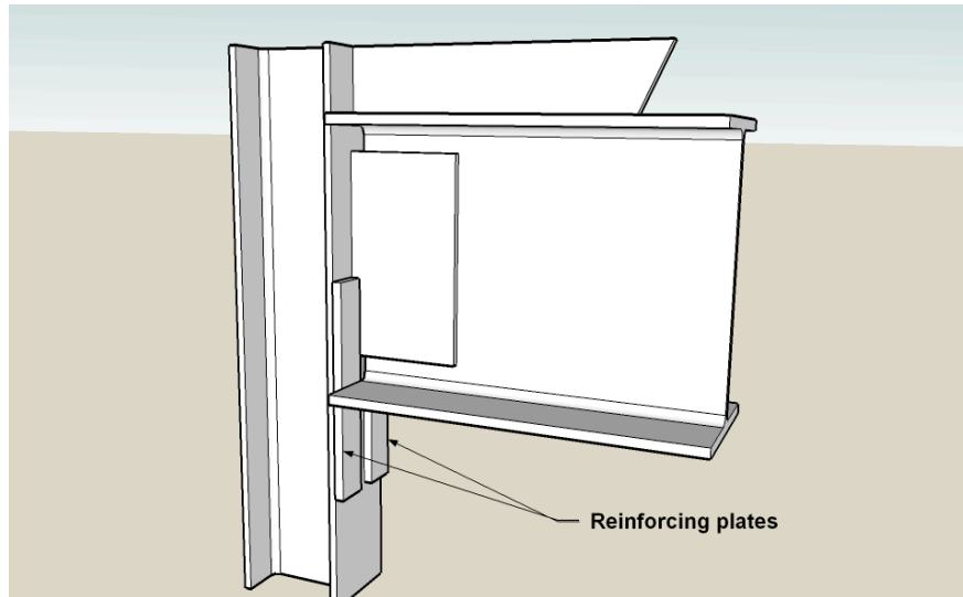
Figure 6.19 Details of reinforcement: reinforcing plates
