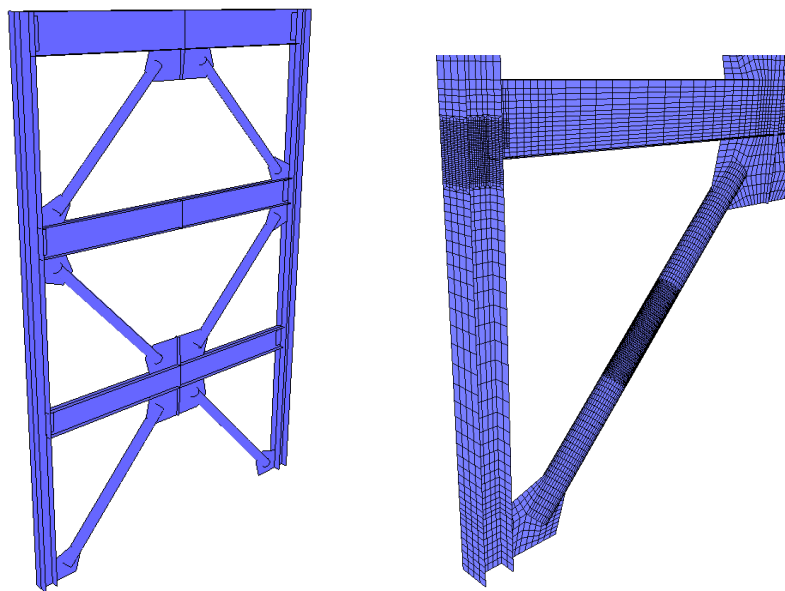
Figure 6.30 Finite element model and refined regions of the building
