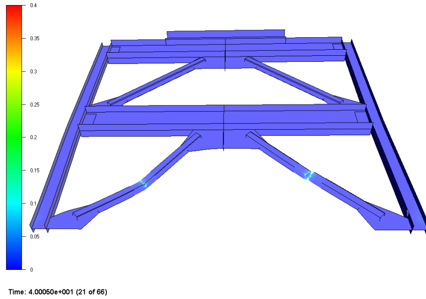
Figure 5.31 Damage and fracture of brace
