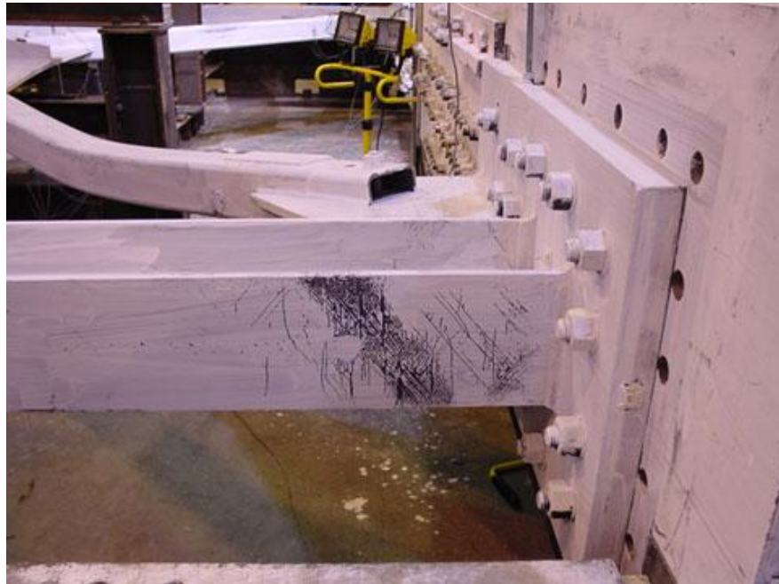
(a) Global buckling
