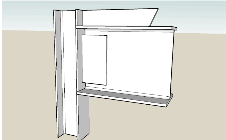
Figure 6.17 Details of reinforcement: reference
