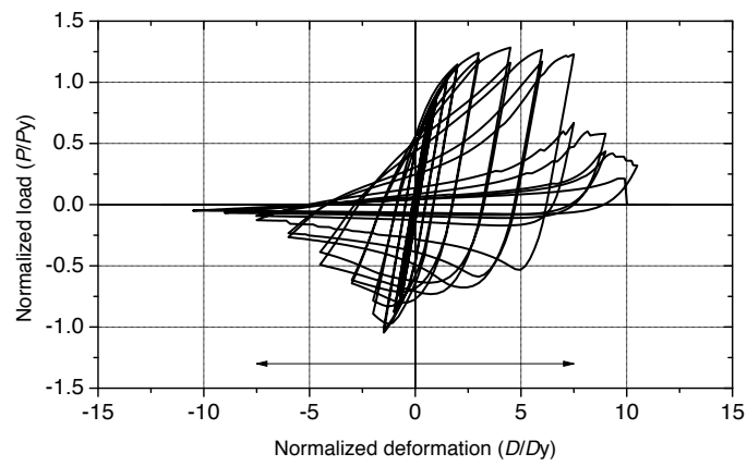
(b) b/t = 14.2
