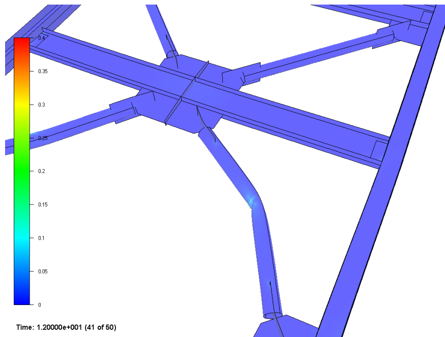
Figure 6.28 Analysis result of in-plane buckling of braces
