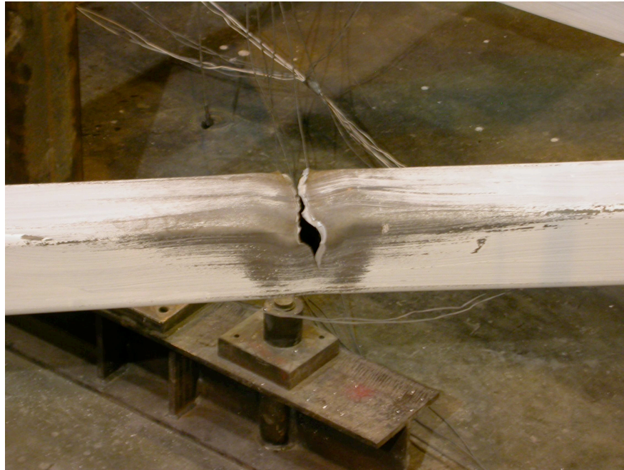
(a) Crack propagation
