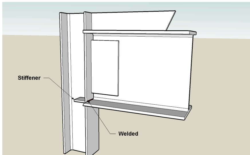
Figure 6.22 Details of reinforcement: stiffener and welded flanges
