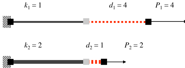
Figure A.4 A linear example
