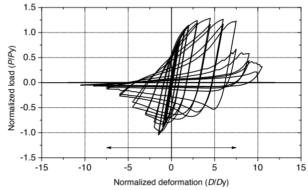
(b) KL/r = 51
