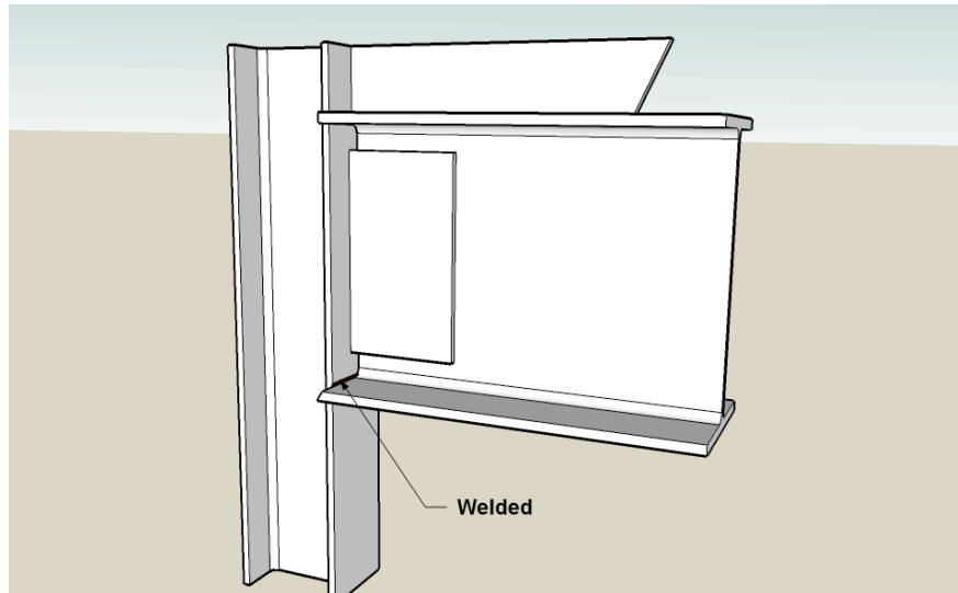
Figure 6.21 Details of reinforcement: welded flanges
