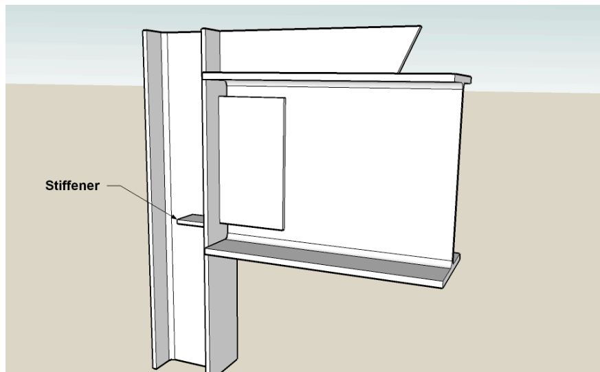
Figure 6.18 Details of reinforcement: stiffener
