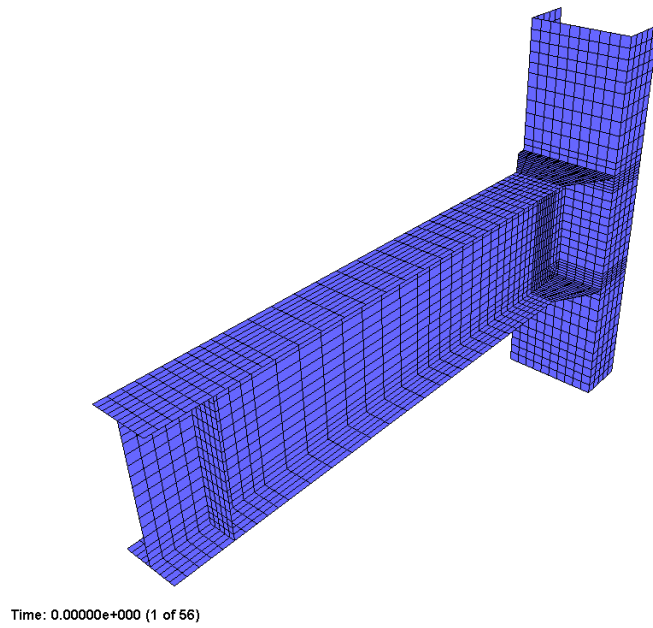
Figure 5.22 Finite element modeling of BW10 specimen
