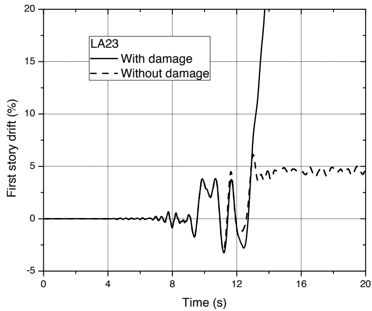
Figure 5.40 First-story drift time history
