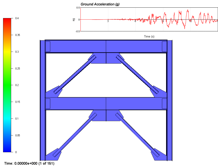
Figure 5.35 Subassembly model and ground motion
