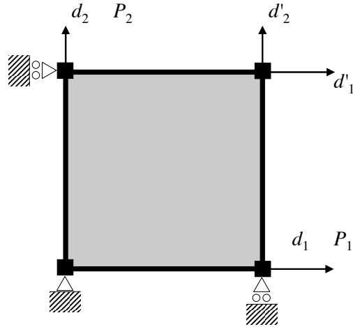
Figure A.9 Biaxial tension of a shell element
