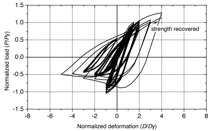
(a) b/t = 14.9 , pass
