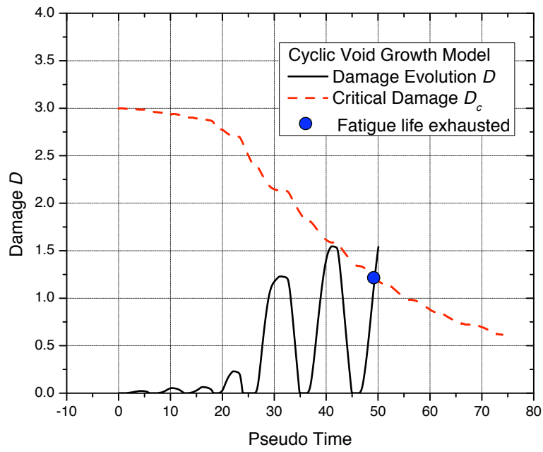
Figure 3.6 Damage evolution of CVGM model
