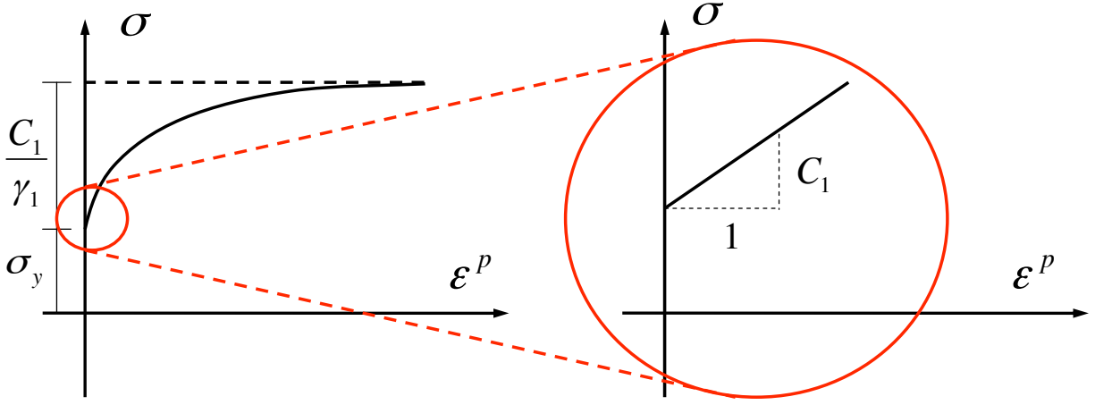
Figure 5.1 Illustration of kinematic hardening parameters
