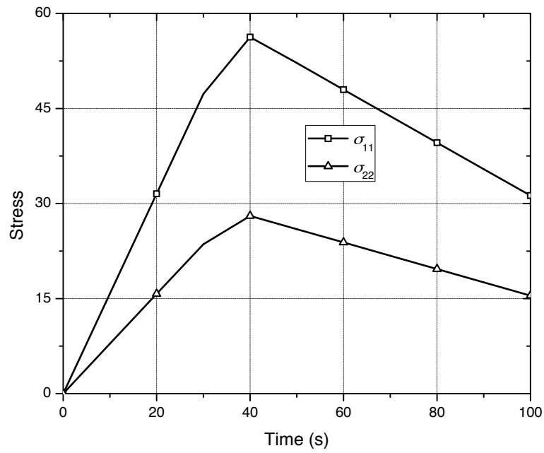
Figure A.11 Stress histories of nonlinear material
