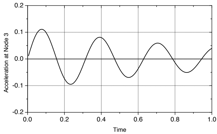
(b) Numerical result, damped, zero mass m_2 = 0
