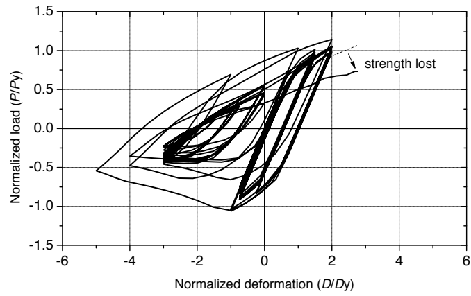
(c) b/t = 17.6 , fail
