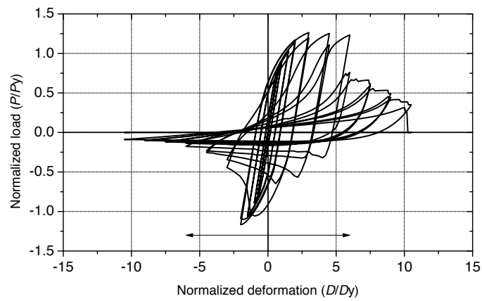
(c) b/t = 28.2
