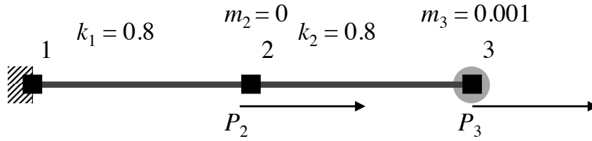
Figure B.1 System for demonstration
