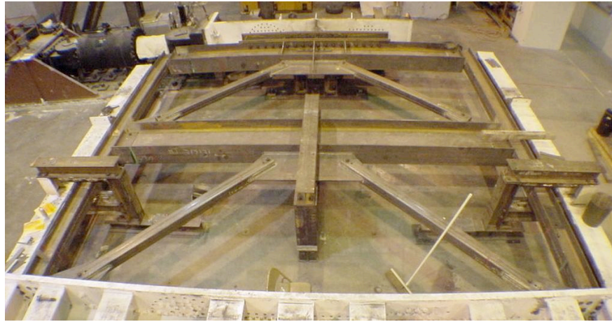
Figure 2.3 Test setup for SCBF (Uriz, 2005)
