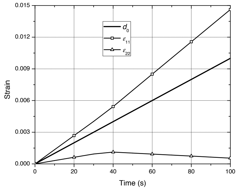
Figure A.10 Strain histories of nonlinear material
