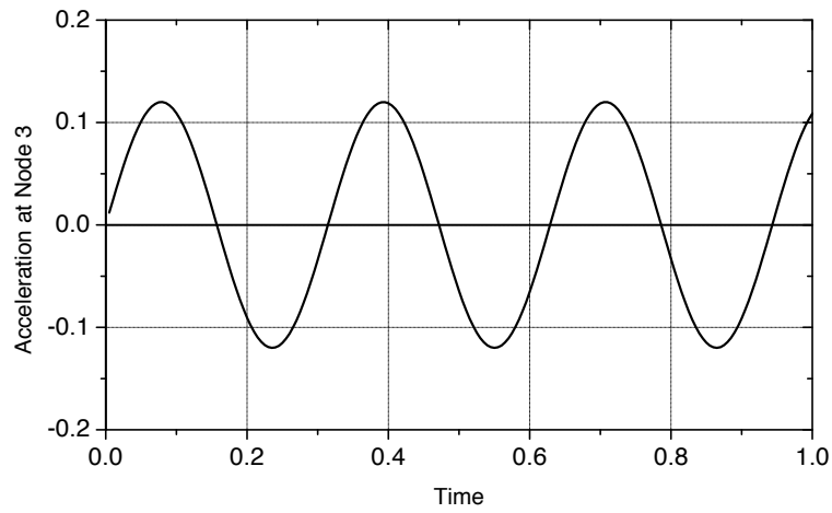
(b) Numerical result, zero mass m_2 = 0
