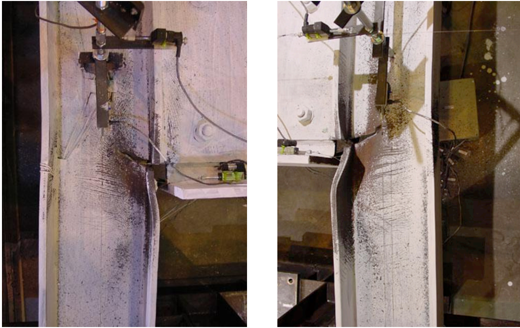
Figure 2.7 Beam-column connection failure (Uriz, 2005)
