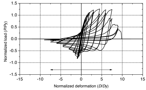
(c) KL/r = 70
