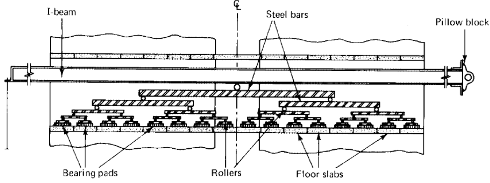
Figure A.1 Whiffle-Tree load system (Harris and Muskivitch, 1980)
