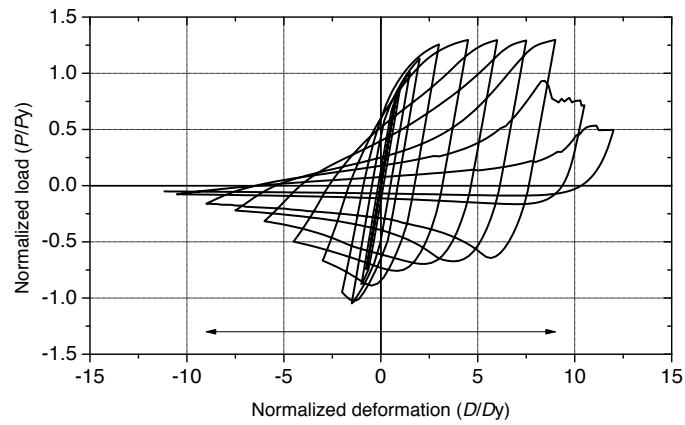
(a) 1 cycle per deformation level
