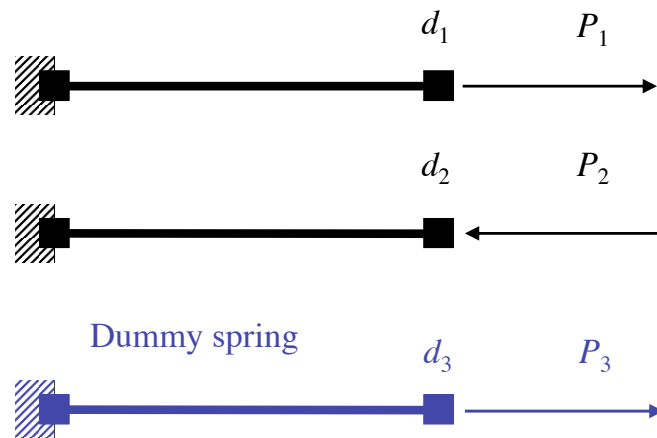
Figure A.14 A two-spring system and a “dummy” spring
