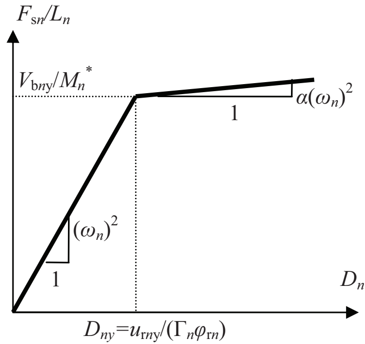
(b) Force-deformation curve for n th-mode SDF system
