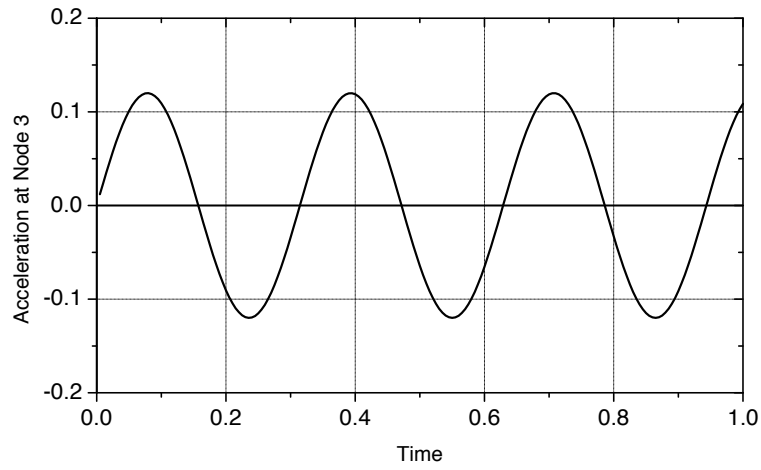
(a) Numerical result, undamped, zero mass m_2 = 0
