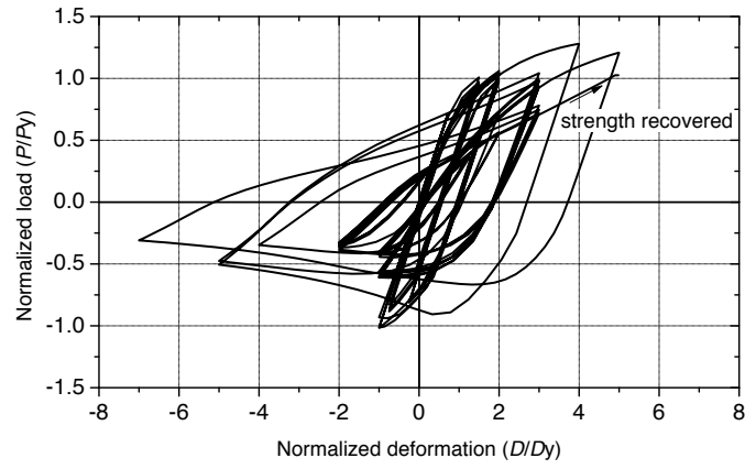
(a) b/t = 12.5 , pass
